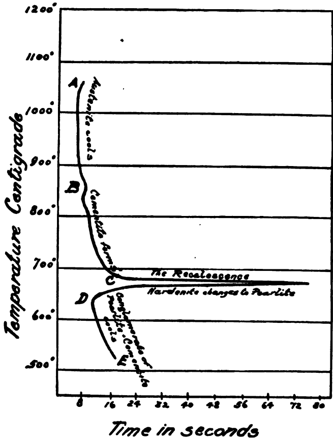
Fig. 69. Retardations in the Undisturbed Cooling of Hard Steel of 1.25 per cent Carbon.
